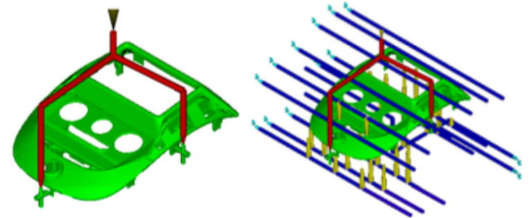
Feed system with Part
